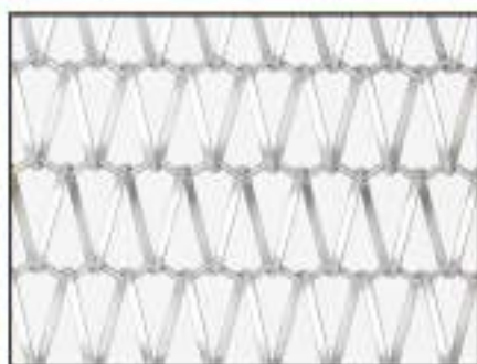
Material: SS201, 302, 304, 316 Cross/Spiral diameter: 2.0mm/1*2.5mm Cross/Spiral pitch: 25mm/12mm
