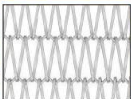
Material: SS201, 302, 304, 316 Cross/Spiral diameter: 3.0mm/1*6mm Cross/Spiral pitch: 70mm/25mm
