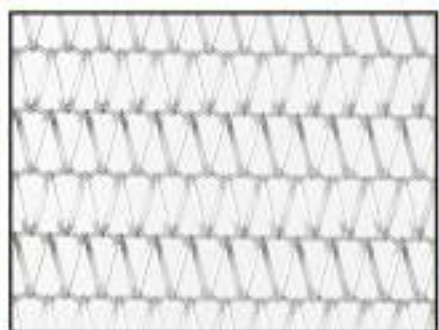
Material: SS201, 302, 304, 316 Cross/Spiral diameter: 1.5mm/1*1.7mm Cross/Spiral pitch: 17mm/8mm
