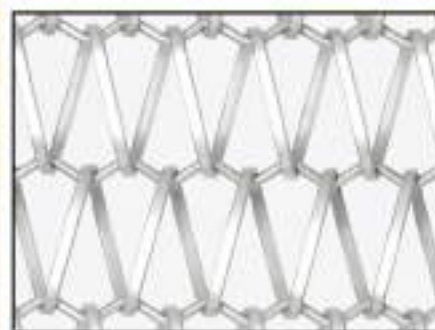
Material: SS201, 302, 304, 316 Cross/Spiral diameter: 2.0mm/1*4mm Cross/Spiral pitch: 30mm/15mm
